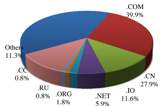
TLD Distribution of the Malware-hosting Websites' Domains (Apr 1-Apr 7)
